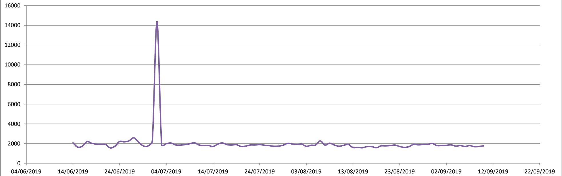
Retail ebanking interface PISP Average Time Taken in milliseconds
